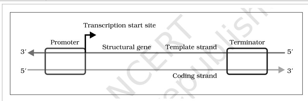
Figure 5.9 Schematic structure of a transcription unit. The Promoter lies upstream with the Transcription start site arrow on it, then the Structural gene , and the Terminator downstream; the upper strand runs 3' to 5' and is the Template strand , the lower runs 5' to 3' and is the Coding strand .
