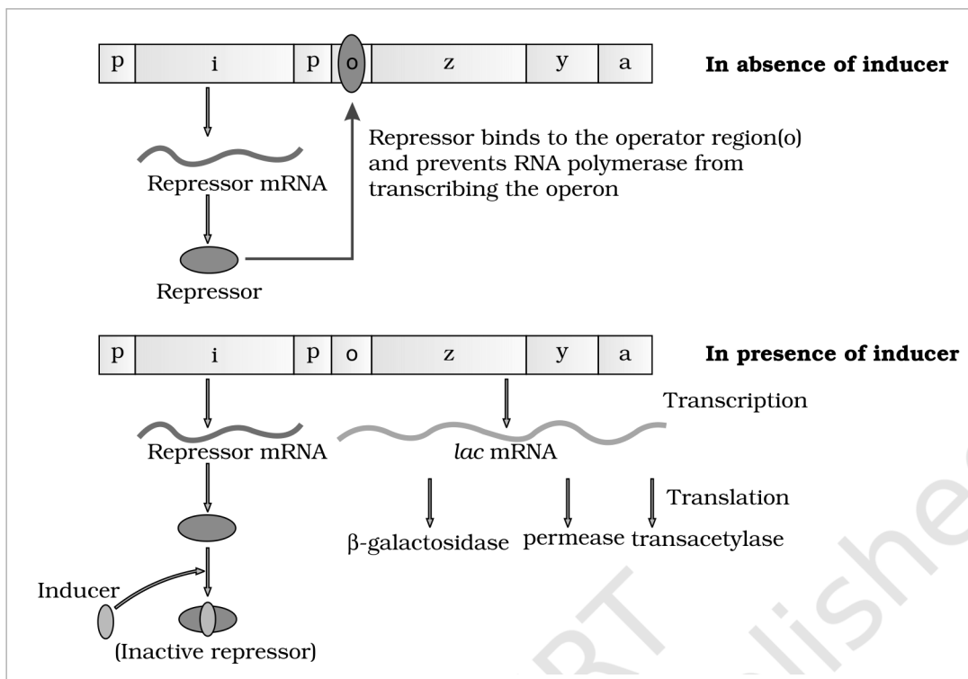
Figure 5.14 The lac operon. In absence of inducer , the Repressor mRNA from the i gene gives the Repressor , and the Repressor binds to the operator region ( o ) and prevents RNA polymerase from transcribing the operon. In presence of inducer , the Inducer gives an Inactive repressor , so lac mRNA is made and Transcription followed by Translation yields beta-galactosidase , permease and transacetylase .
